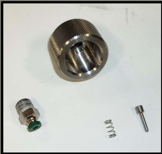
Plug disassembled (shown with 4351 Fitting, standard 1/8")
